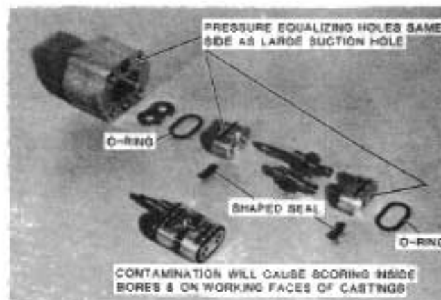
FIG. 11. Pump A1 Disassembled
