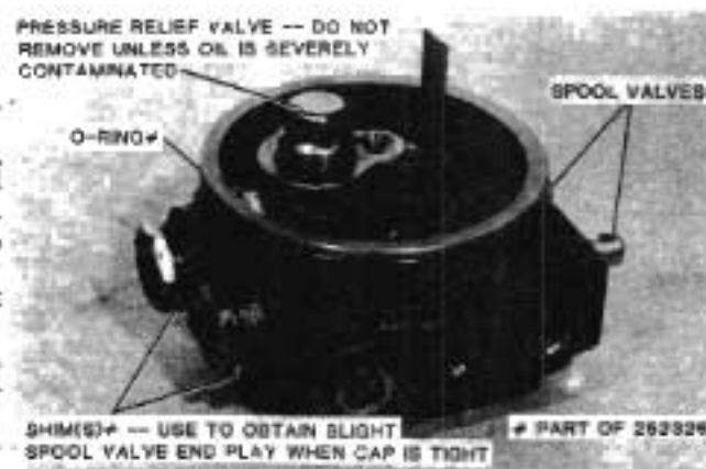
FIG. 20. Dual Hydraulic Valve Body Assembly
