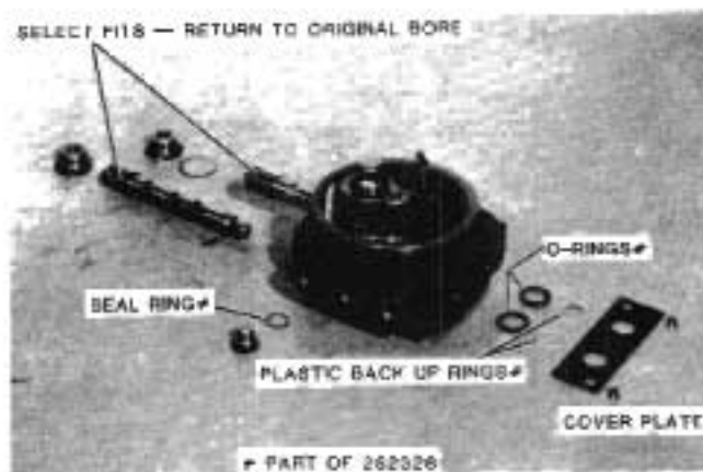
FIG. 21. Dual Hydraulic Spool Valves & Seals
