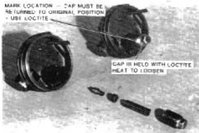
FIG. 19. Pressure Relief Valve
