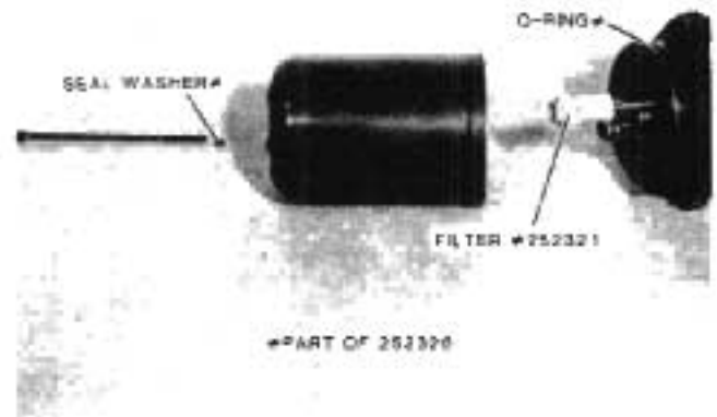
FIG. 7. Dual Hydraulic Unit
