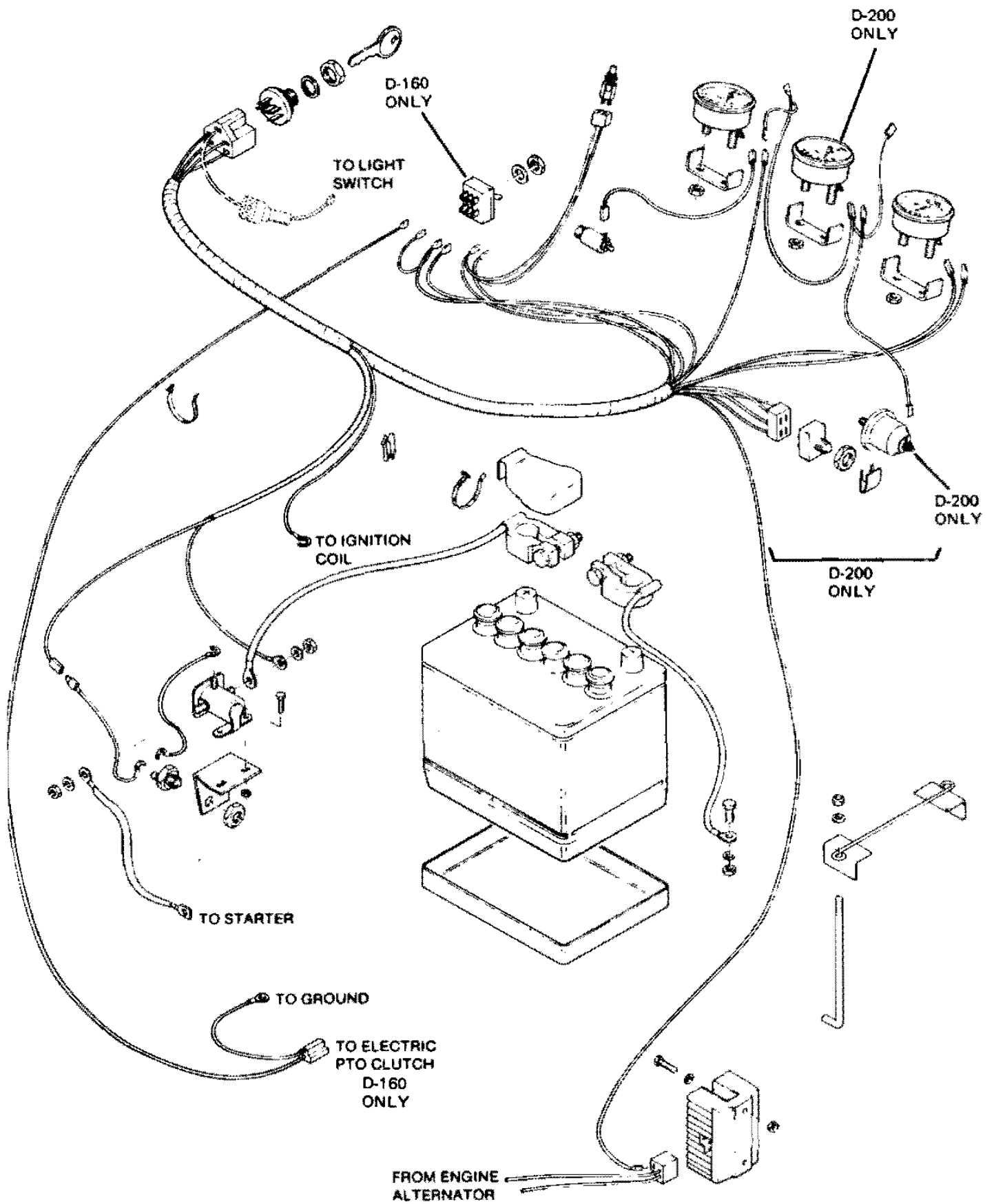
Fig. 6-20 D-Series Harness Routing
