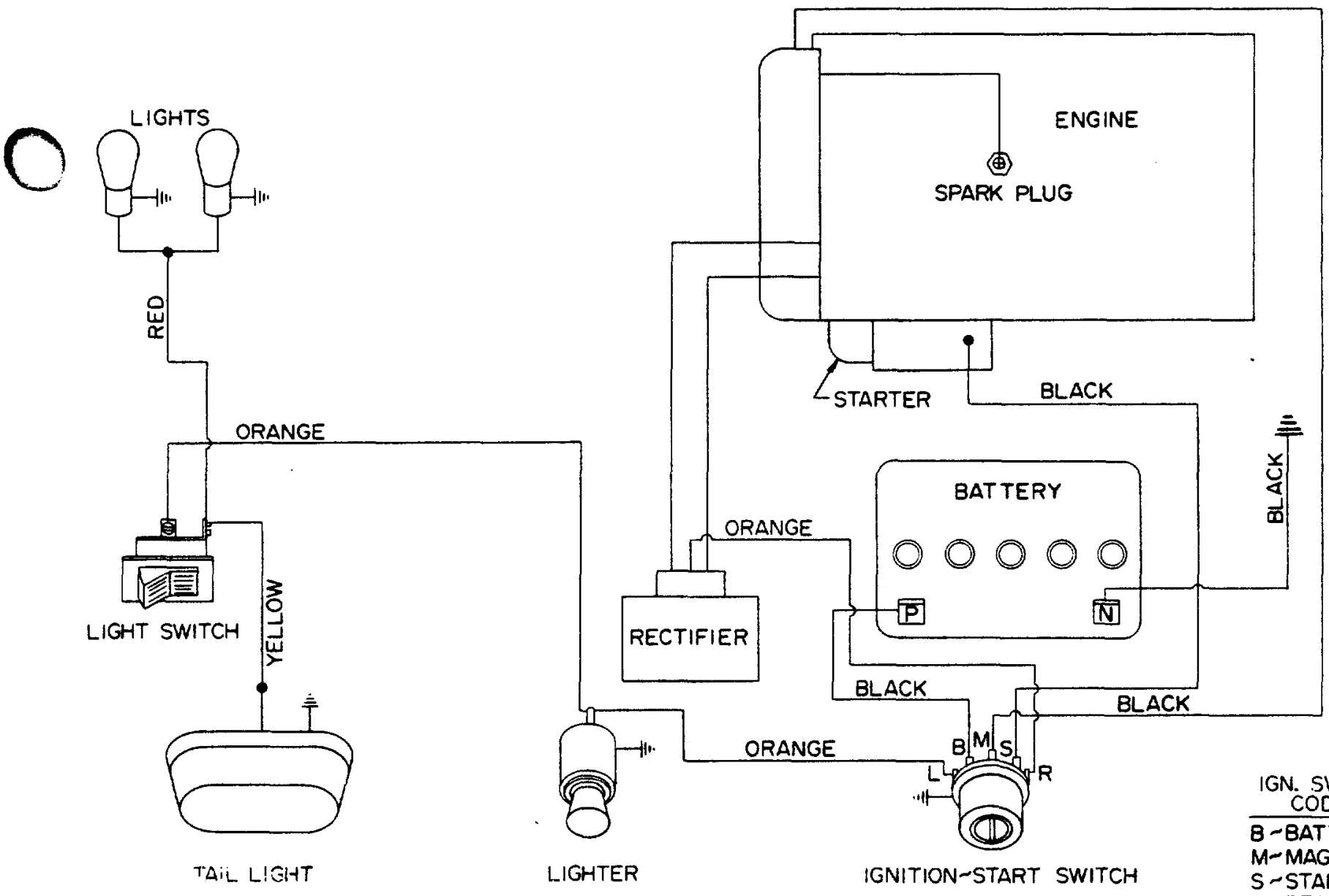
WIRING DIAGRAM
